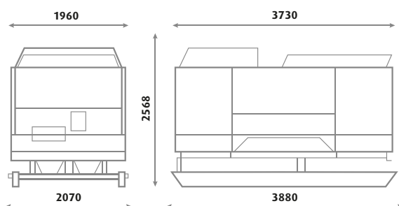
Skid mount
