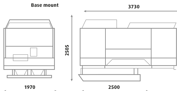
Base mount
